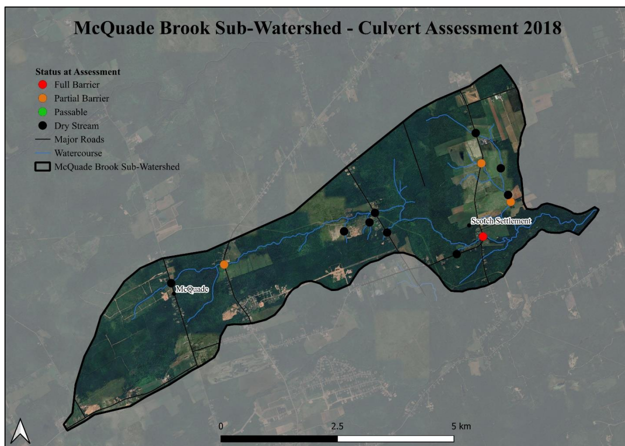
Figure 65: Culvert assessment results of the McQuade Brook sub-watershed, 2018.
