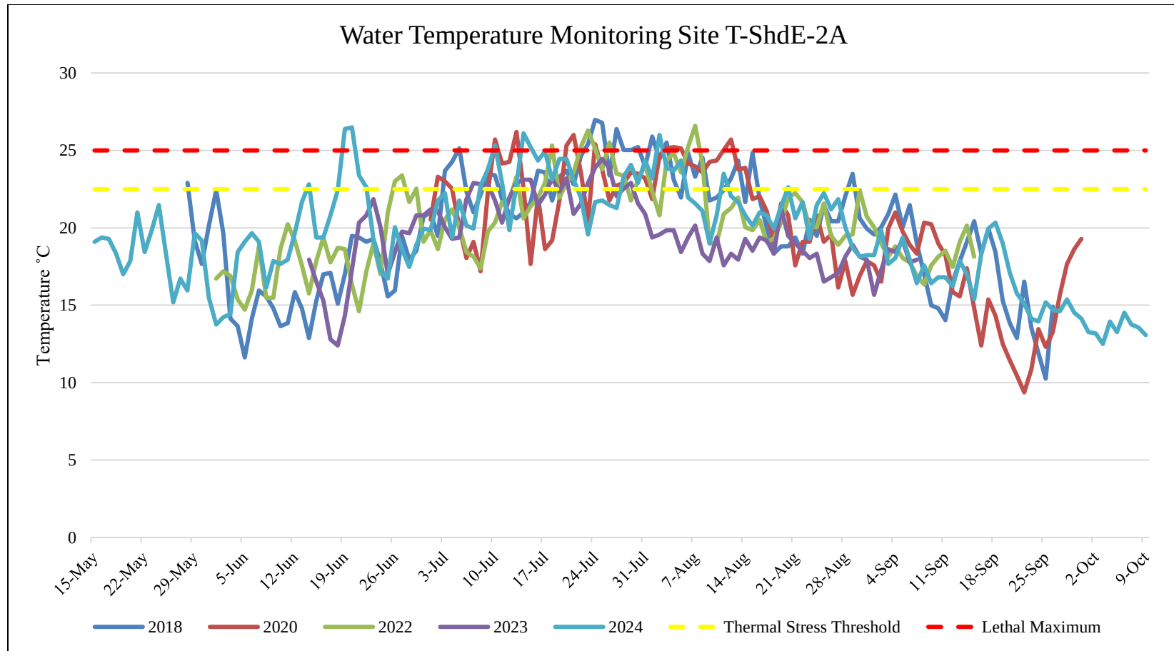
Figure B 6: Thermograph chart for monitoring station T-ShdE-2A, Shediac River 2018-2024.
