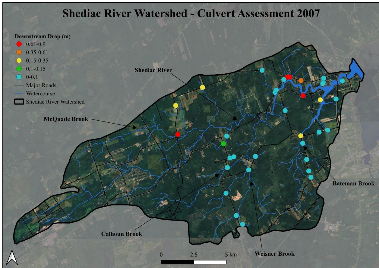
Figure 26: Culvert assessment results from the Shediac River watershed, 2007.
