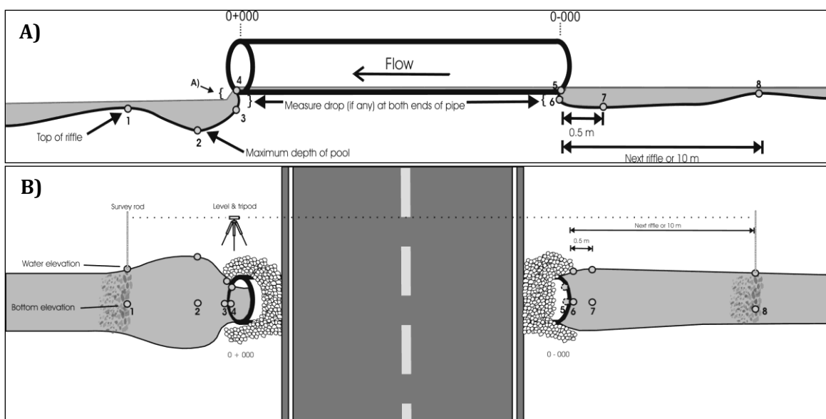
Figure 3: A) Lateral views of culvert assessment measurement locations. B) Aerial view.
