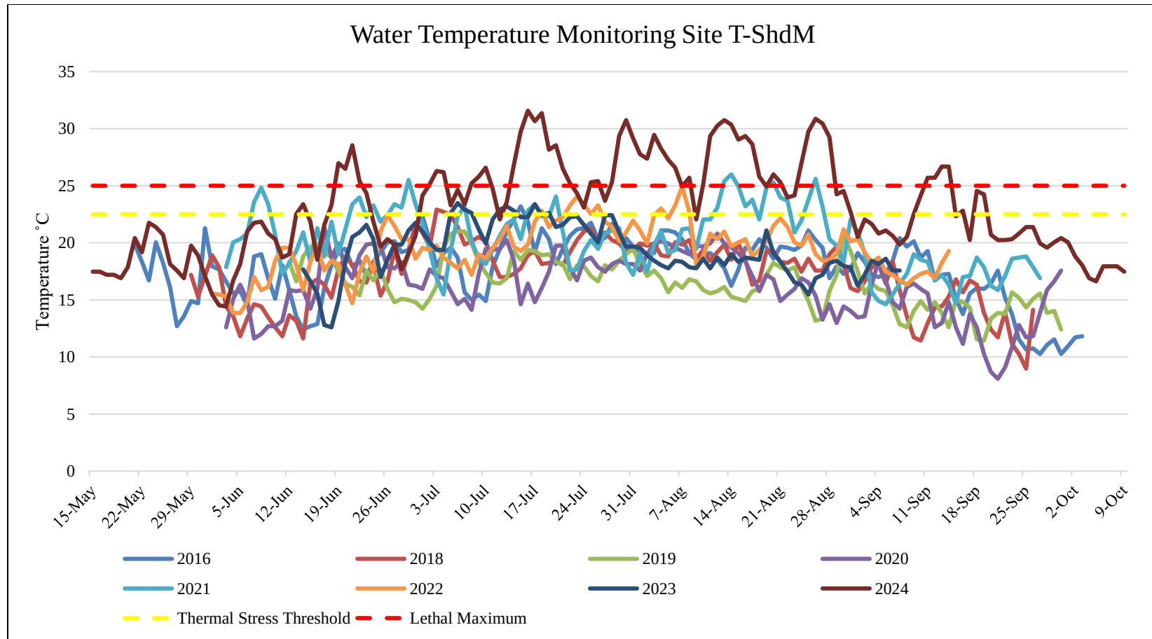
Figure B 7: Thermograph chart for monitoring station T-ShdM, Shediac River 2016-2024.
